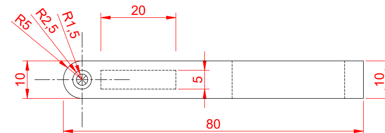
LEFT VIEW
